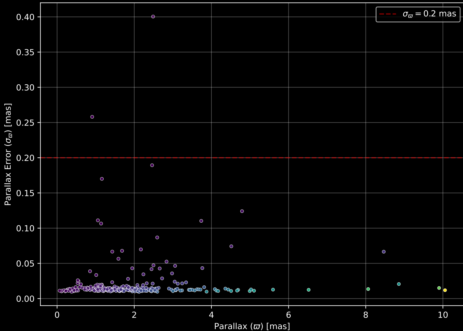
GALAH DR4 Field: [7012] Parallax Quality (n= 303)
