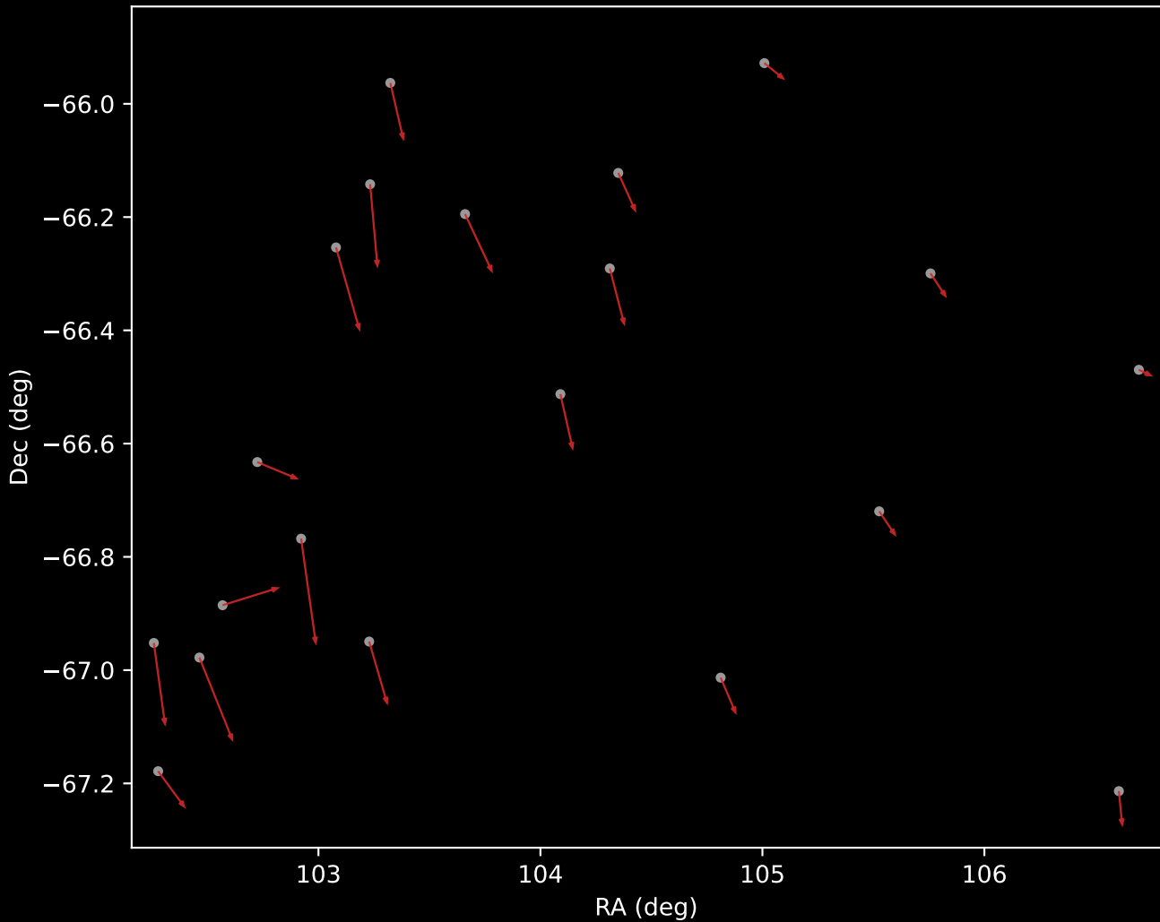
GALAH DR4 Cluster 6 Proper Motion Vectors (n=20)
