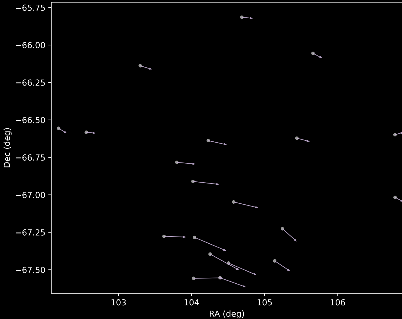
GALAH DR4 Cluster 9 Proper Motion Vectors (n=20)
