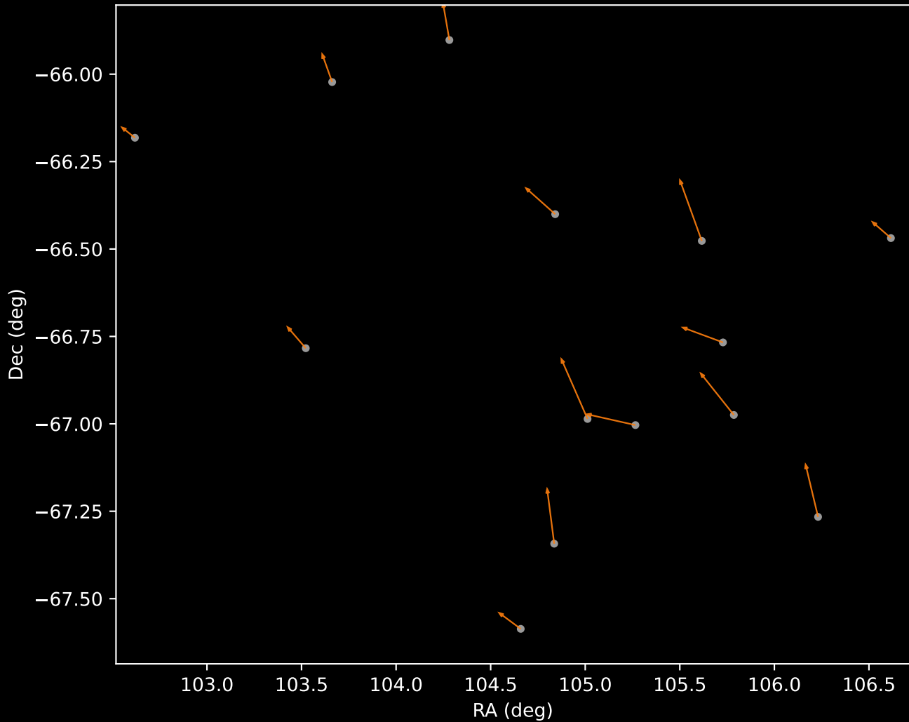
GALAH DR4 Cluster 2 Proper Motion Vectors (n=14)
