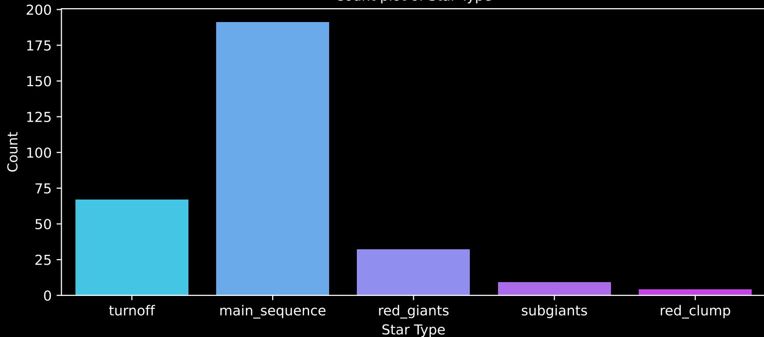
GALAH DR4 Field: [7012] Count plot of Star Type
