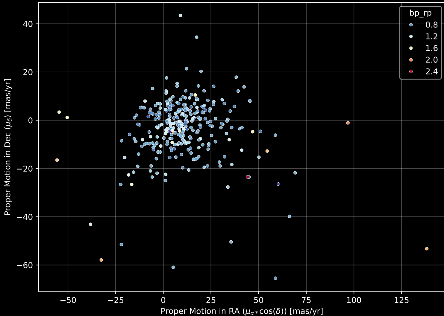
GALAH DR4 Field: [7012] Proper Motion Diagram (n= 303)
