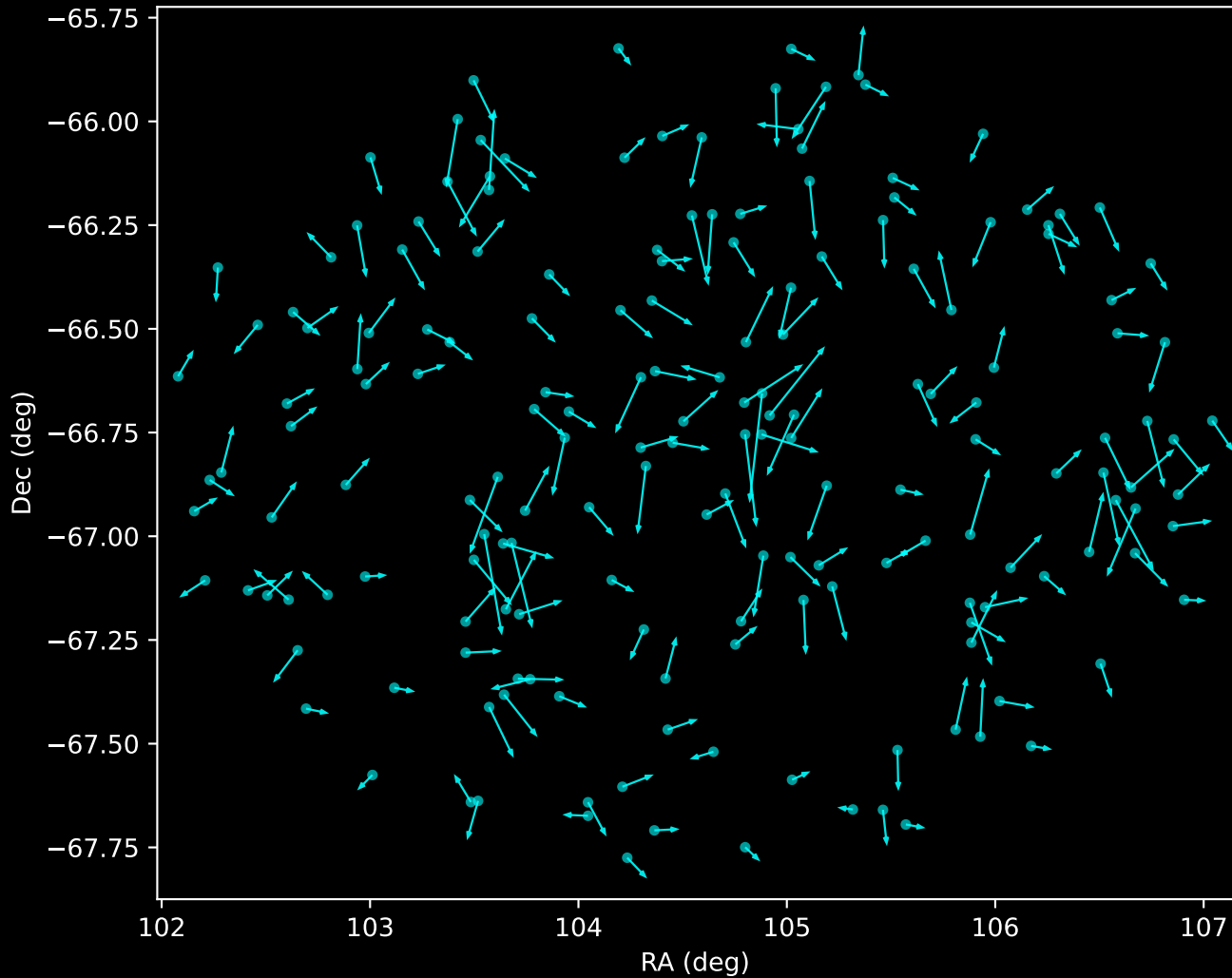
GALAH DR4 Noise Stream Proper Motion Vectors (n=180)
