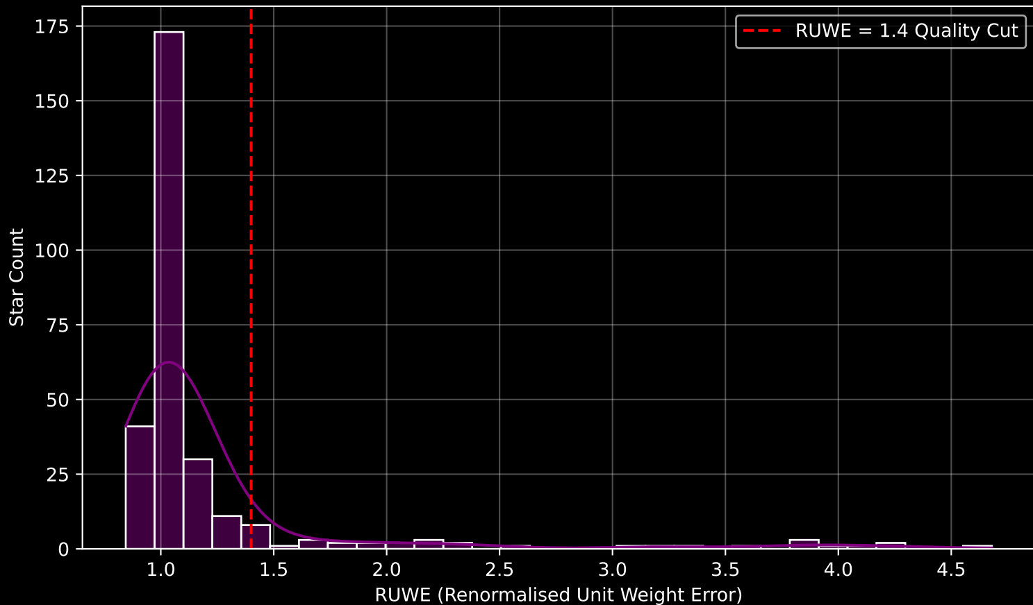
GALAH DR4 Field [7012] RUWE Distribution (n= 291)
